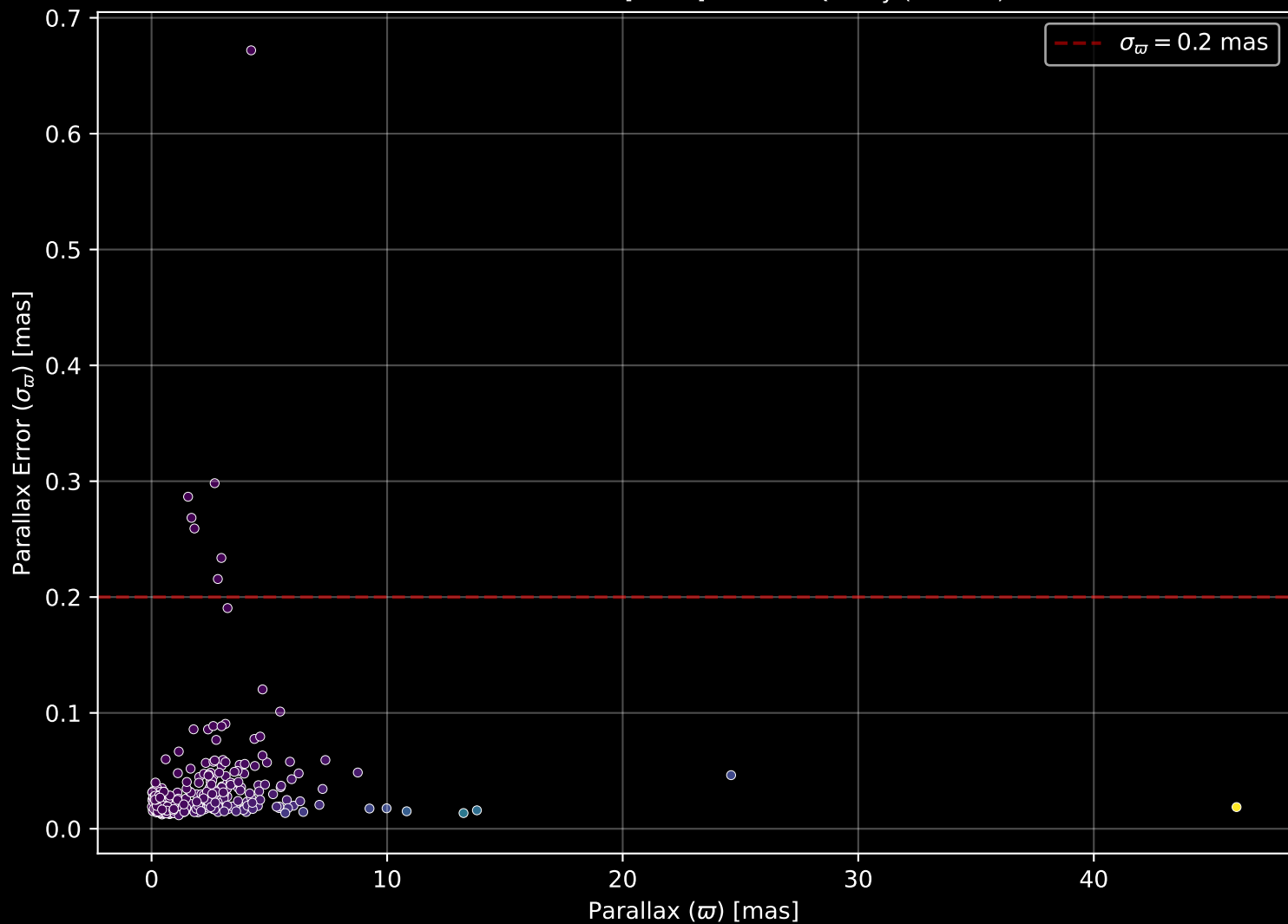
APOGEE DR17 Field: [SGR1] Parallax Quality (n= 373)
