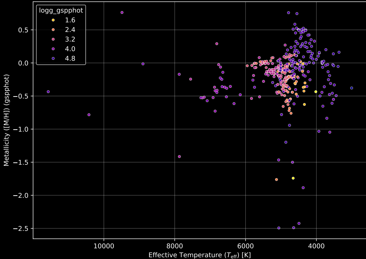
APOGEE DR17 Field: [SGR1] Stellar Population Parameters (n= 373)
