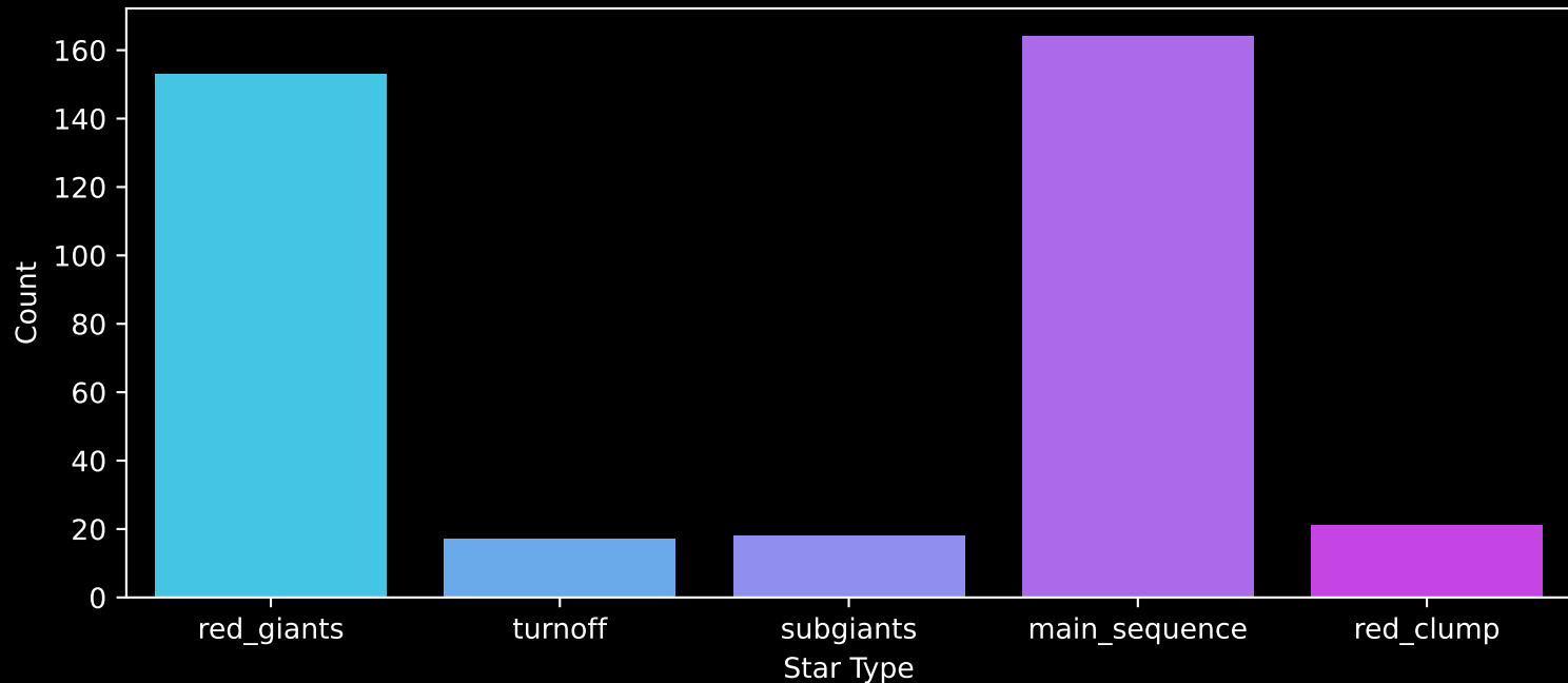
APOGEE DR17 Field: [SGR1] Count plot of Star Type
