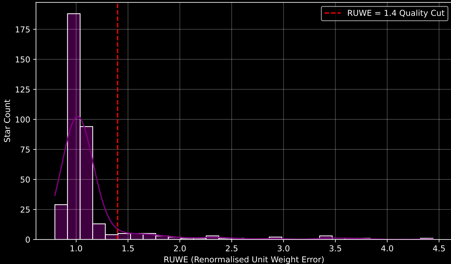
GAPOGEE DR17 Field [SGR1] RUWE Distribution (n= 363)
