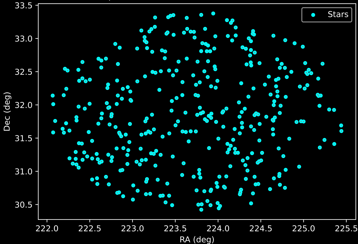
APOGEE DR17 Field: [SGR1] Proper Motion Vectors for Gaia Star Field (n= 373)
