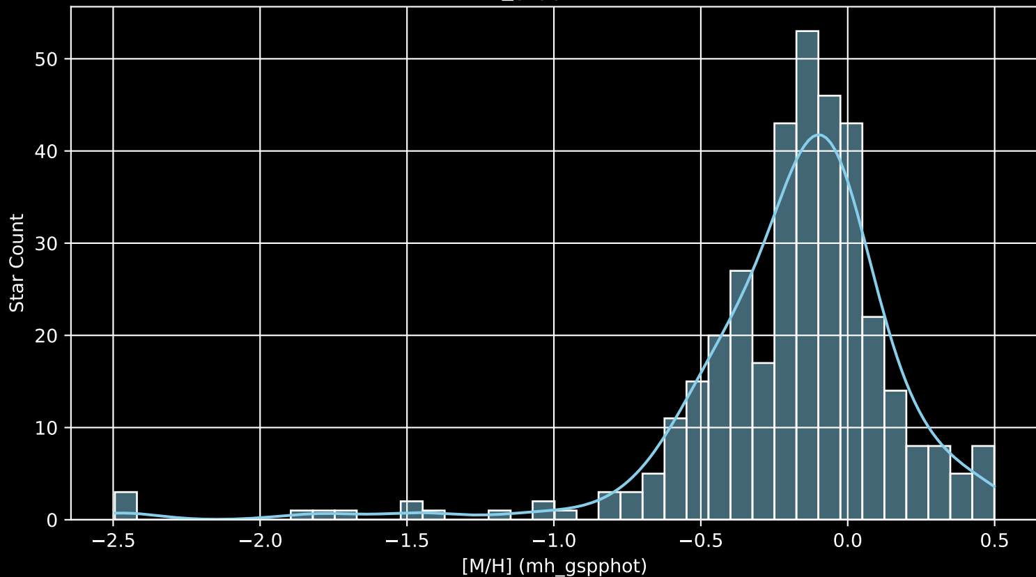
APOGEE DR17 Field: [SGR1 [M/H] (mh_gspphot) (n= 364)
