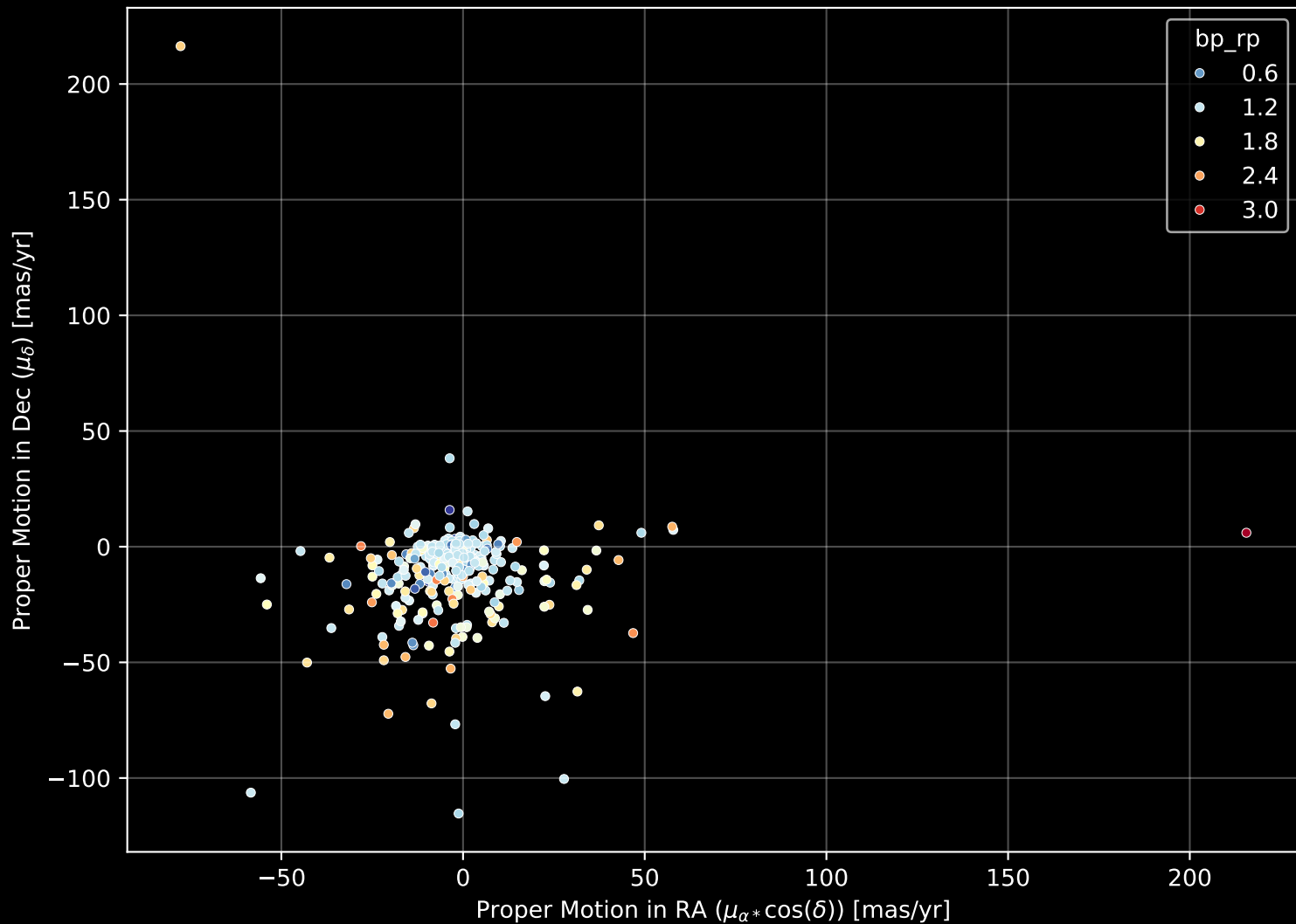
APOGEE DR17 Field: [SGR1] Proper Motion Diagram (n= 373)
