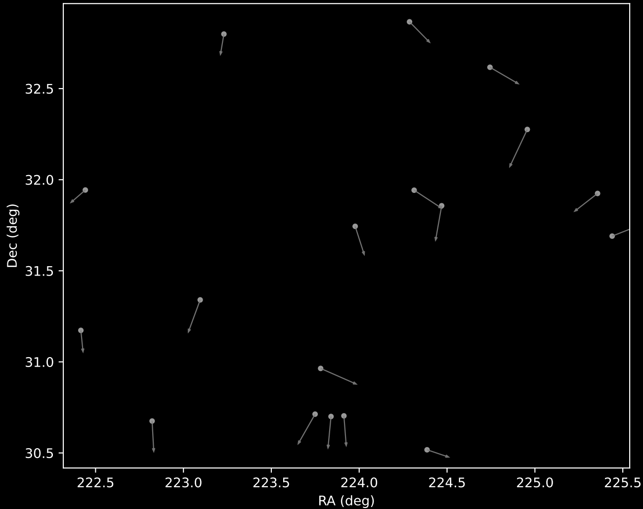
APOGEE DR17 Cluster 14 Proper Motion Vectors (n=18)
